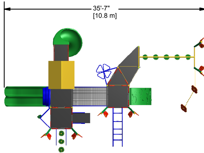
PLAN PLAN VIEW
