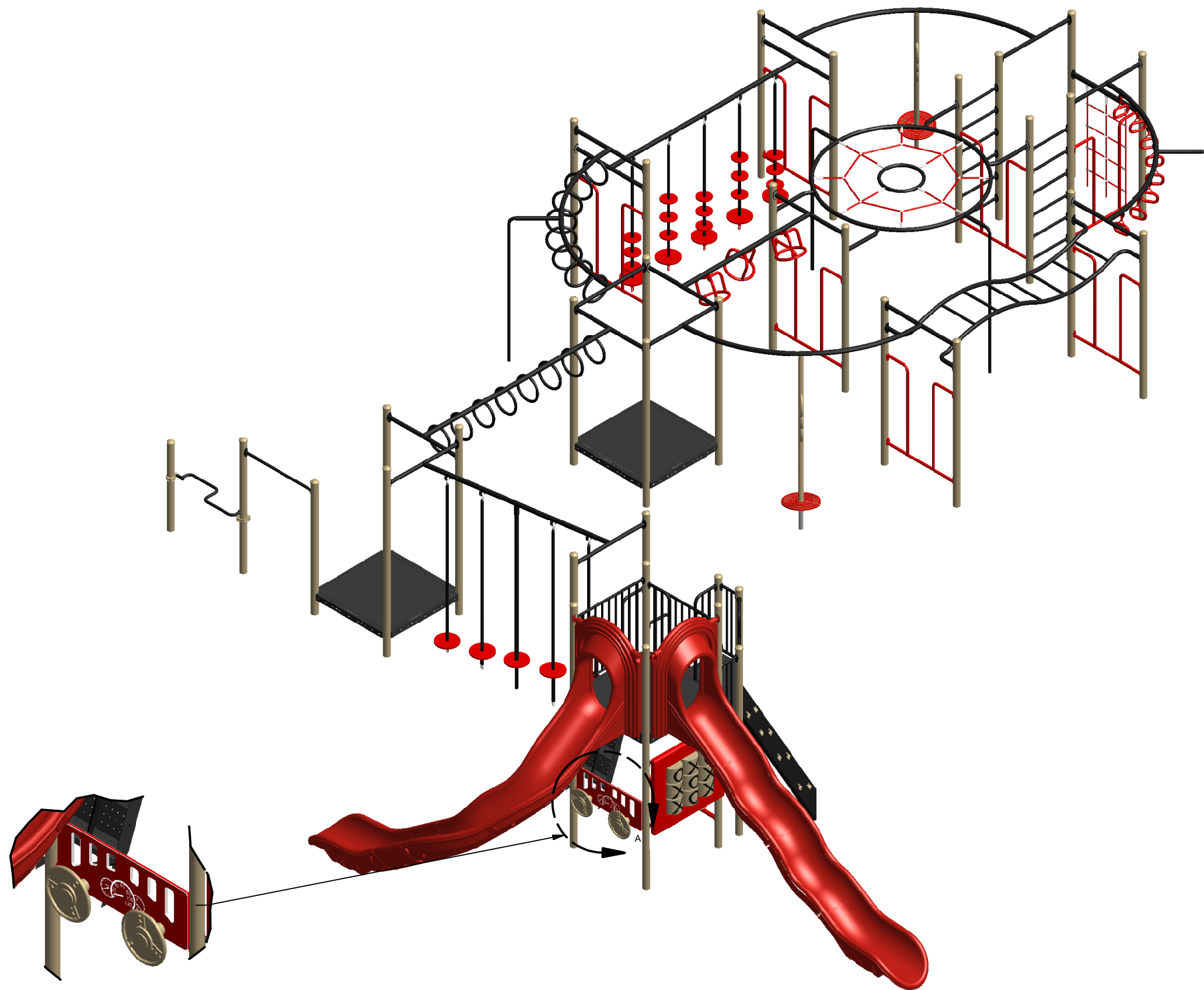
DETAIL A
